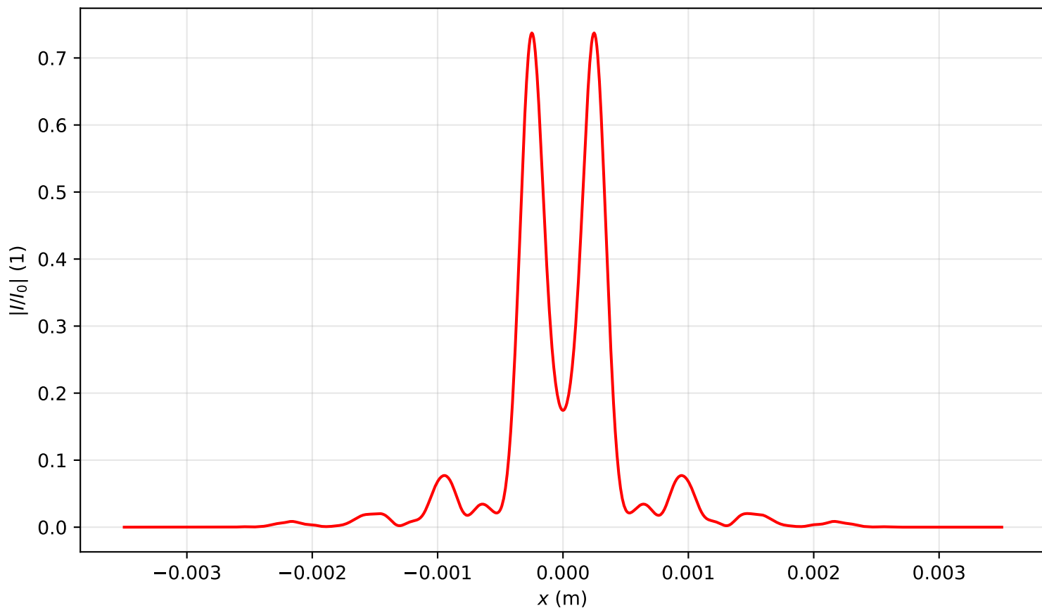
Intensity profile I(x, y = 0, z = 1.911)/I_0 , P_{in}=5.0P_{cr} , artificial time
